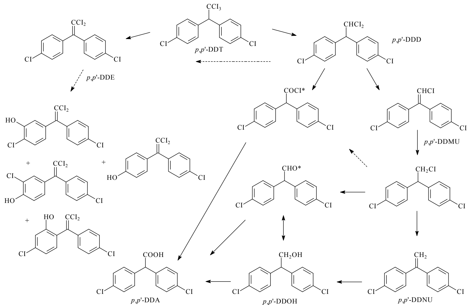
Fig. 4.1 Postulated metabolism scheme of p,p' -DDT in rats
