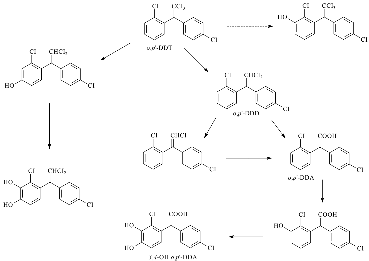
Fig. 4.2 Postulated metabolism scheme of o,p' -DDT in rats
