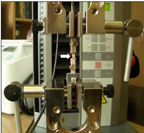
Figure 2.6. Uniaxial testing system Zwick/Roell BDO-FB0.5TS, specially constructed specimen fixator can be seen. Arrow marks the specimen.
