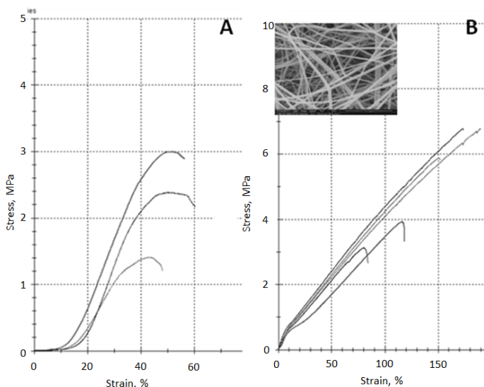
Figure 3.2. Stress/strain curves: A) porcine aortic valve circumferential direction and B) PUR 6.2 g/m 2 . Insert – a scanning electron microscope image of PUR nanofiber material
