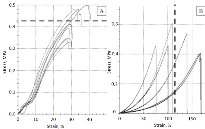
Figure 3.5. Stress/strain curves from a single experiment with nanofiber materials
