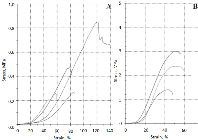
Figure 3.1. Stress/strain curves of porcine valve leaflets from selected experiments: A) radial and B) circumferential direction
