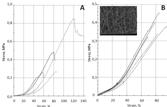
Figure 3.3. Stress/strain curves: A) porcine aortic valve circumferential direction and B) gelatin 5.7 g/m 2 . Insert – a scanning electron microscope image of gelatin nanofiber material
