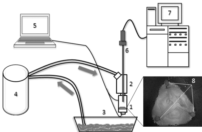
Figure 2.4. A schematic representation of the test setup used in this experiment
