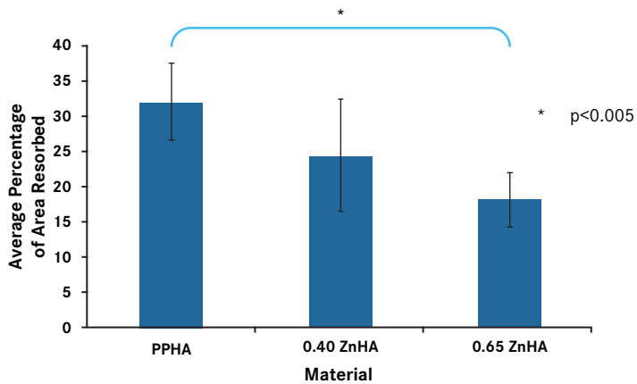
Figure 2. Effect of zinc on the resorption activity of osteoclasts after 21 days.
