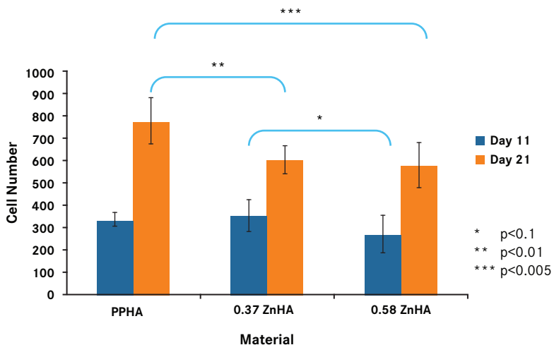
Figure 1. Graph showing effect of zinc on the number of osteoclasts after 11 and 21 days.
